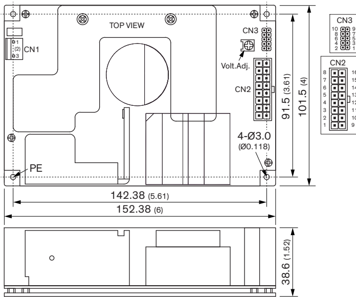
Dimensions in mm (inch) Tolerances: ±0.5 (±0.02)
