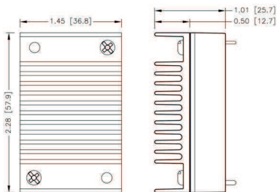
Dimensions in inch, [ ] = mm
