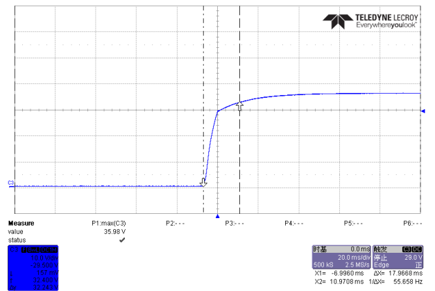
Typical Output Rise Characteristic at 230 Vin
