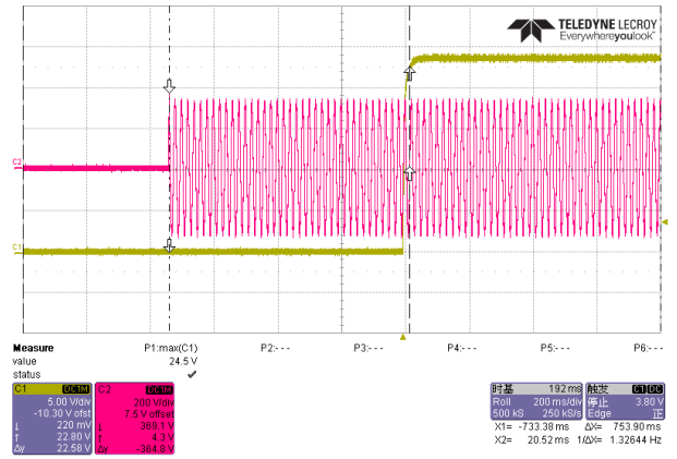
Typical Start-Up Characteristic at 230 Vin
