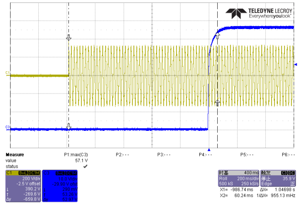
Typical Start-Up Characteristic at 230 Vin
