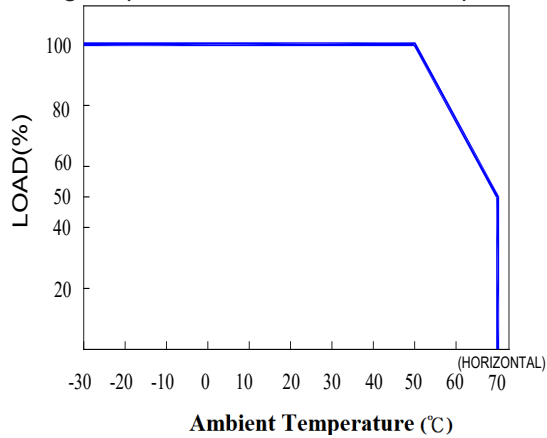
Derating Output Load versus Ambient Temperature
