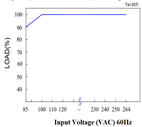
Derating Output Load versus Input Voltage
