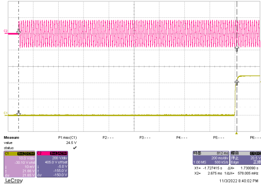
Typical Start-Up Characteristic at 115 Vin
