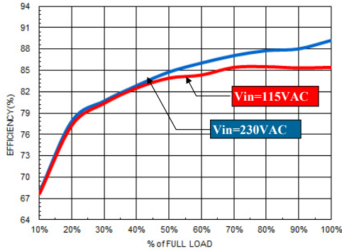
Efficiency versus Output Load
