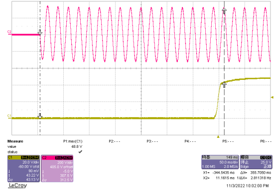
Typical Start-Up Characteristic at 230 Vin
