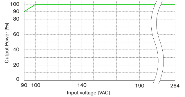
Derating Output versus Input Voltage
