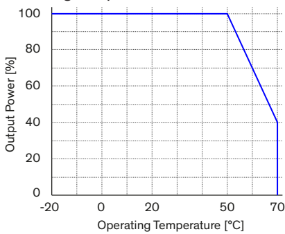
Derating Output versus Ambient Temperature
