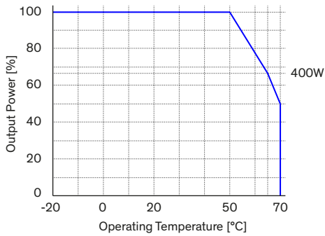
Derating Output versus Ambient Temperature
