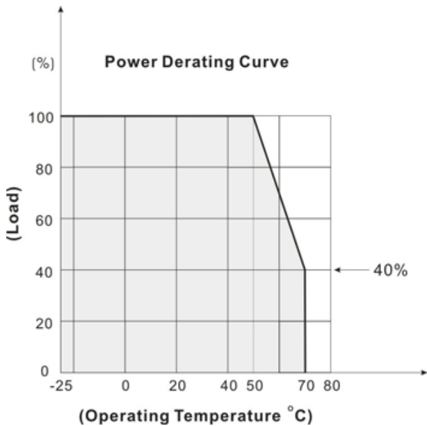
Derating Output Load versus Ambient Temperature
